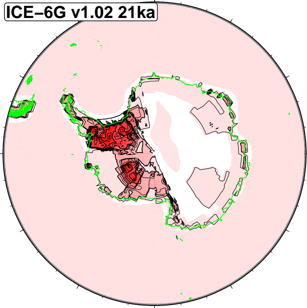
Diff. from present (km)
