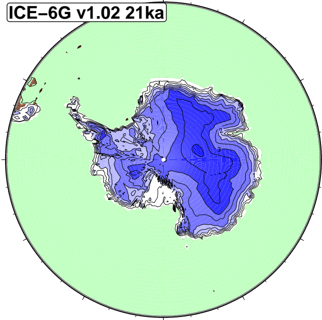
Surface elevation (km)
